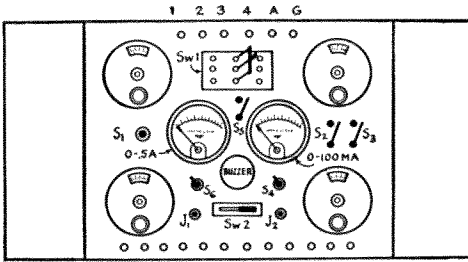
Showing arrangements of switches, meters, and jacks in circuit diagram of Fig. 2
